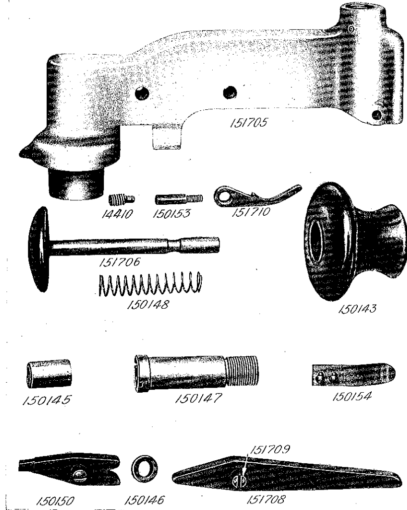
OPERATING HANDLE, CAT. NO. 34343
